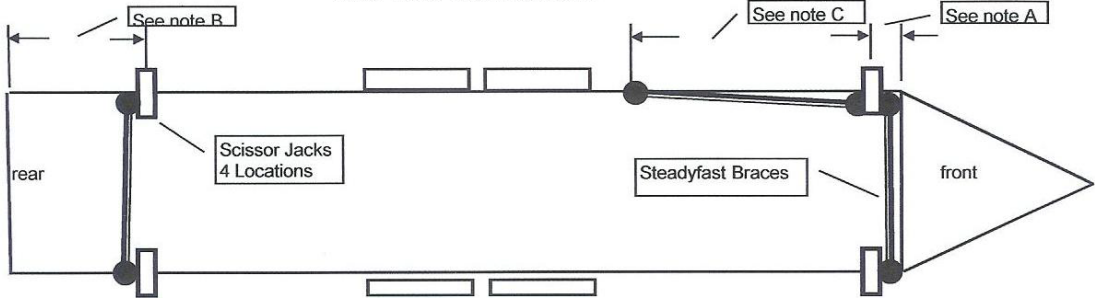
FIGURE 2 Travel Trailer Brace Locations
