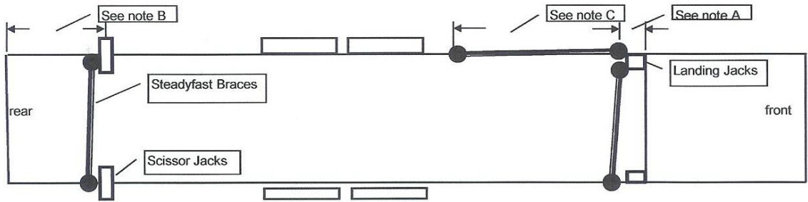
FIGURE 1 Fifth Wheel Brace Locations
